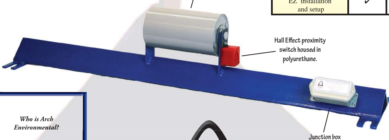
CEMA Scale Duty Idler
