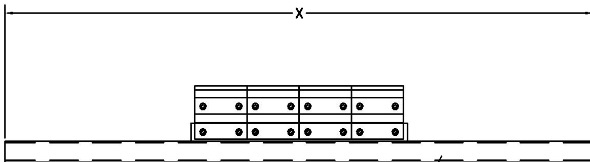
2 3/8 OD (SCH 80) PIPE FRAME LENGTH OF FRAME CAN BE FIELD ALTERED IF REQUIRED
